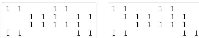
Figure 6.2: Left: A matrix having the 2-C1P, but not the 2-XC1P. Right: A matrix having the 2-XC1P. In all figures of this chapter, only the 1-entries in matrices are displayed (that is, all 0-entries are omitted).
