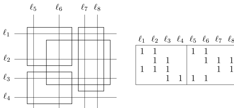
Figure 6.2: Left: A matrix having the 2-C1P, but not the 2-XC1P. Right: A matrix having the 2-XC1P. In all figures of this chapter, only the 1-entries in matrices are displayed (that is, all 0-entries are omitted).
